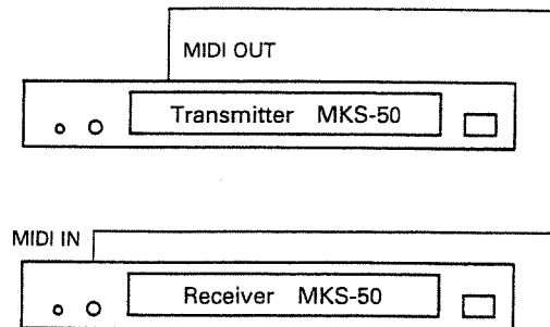
One-way Connection
