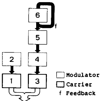
Fig. 5. DX1 Algorithm 1
