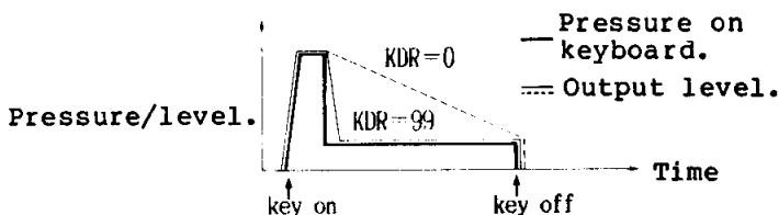
Fig. 69. Decay Rate
