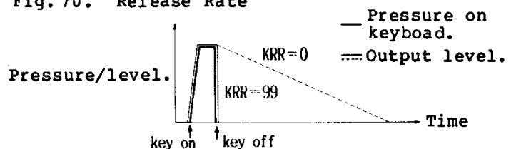
Fig. 70. Release Rate
